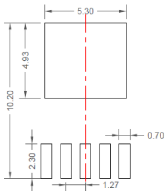
PCB Layout (Recommended)
